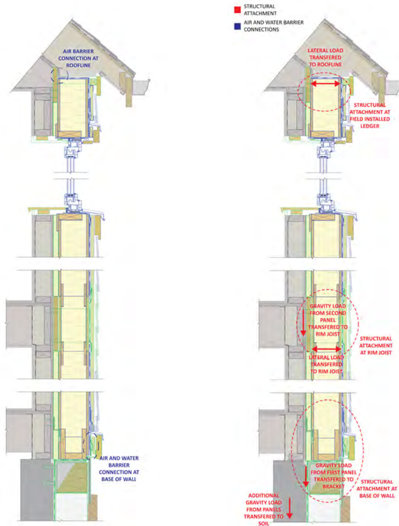
Figure 3-4: Typical structural attachment locations and air barrier connections
