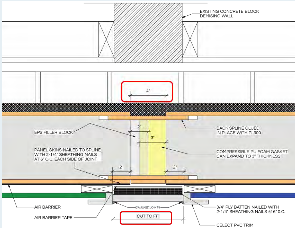
Figure 8-4: Vertical panel joint
